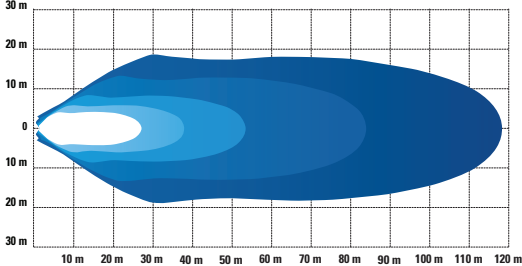
1800 LUMEN FAR FLOOD
