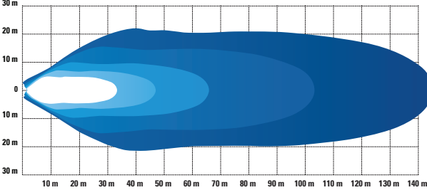
2800 LUMEN FAR FLOOD
