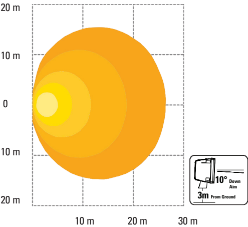
NEAR FLOOD - ISOLUX (64V41-3, 64V51-3)
