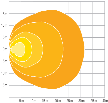
NEAR FLOOD - ISOLUX (64V81-3, 64V91-3, 64V81-4, 64V91-4)
