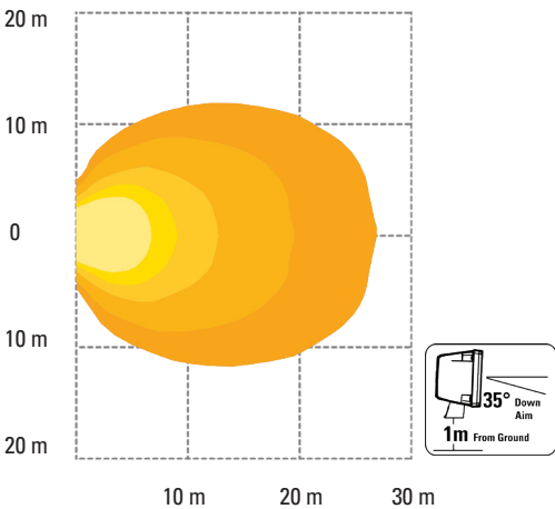
FAR FLOOD (R23) - ISOLUX (64V21-3, 64V31-3)
