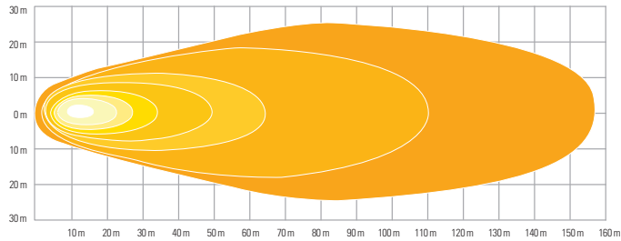
FAR RANGE - (64T31 & 64T61)
