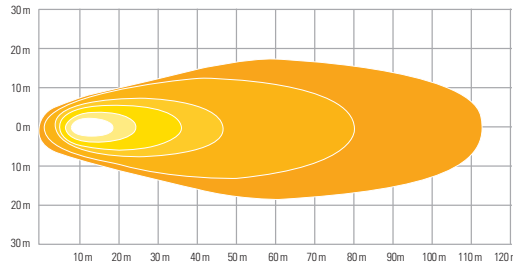
FAR RANGE - (64L31 & 64L61)
