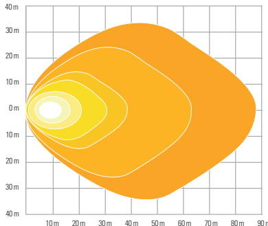
CLOSE RANGE - (64T41 & 64T71)
